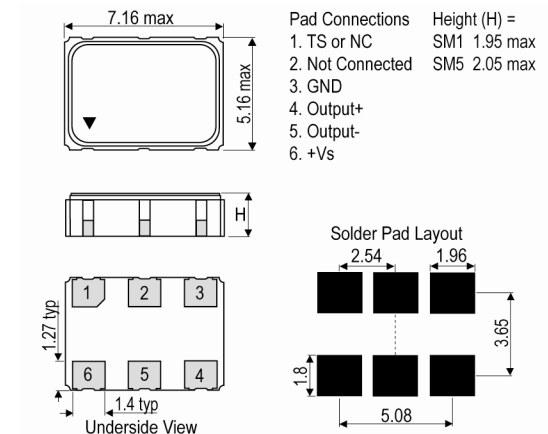
Outline (mm) -SM1 = (Gold plated, RoHS compliant)
