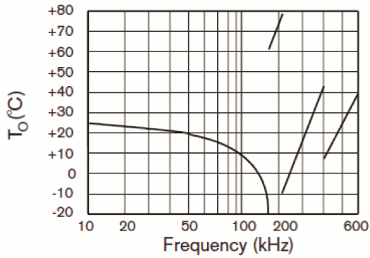
CX1H Typical Turning Point Temperature
